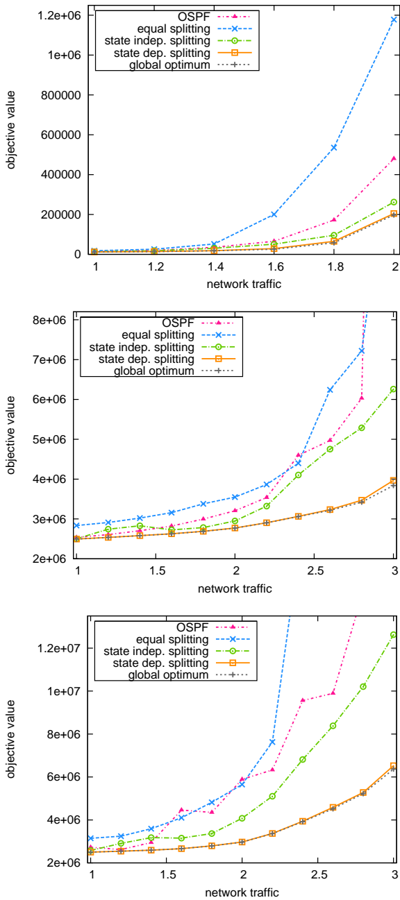
Figure 2: From top to bottom the traffic engineering objective as a function of an increasing traffic load in the hierarchical topology hier50a, tier-1 topology with single edge failures, and mboxtier-1 topology with SRLGs, respectively. The performance of the optimal solution and state-dependent splitting is nearly identical.
